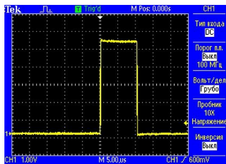
Fig. 5. The form of the output signal
