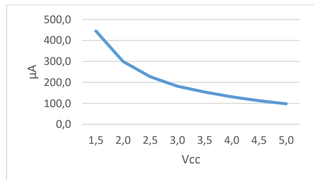
Fig. 2. Quiescent current with snubber circuit.
