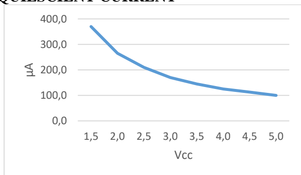
Fig. 1. Quiescent current without snubber circuit.
